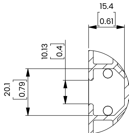
T-Slot DETAIL A SCALE 1:1
