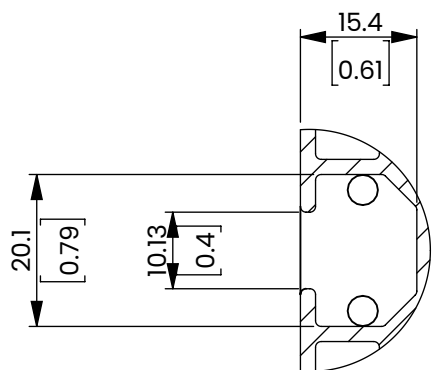
T-Slot DETAIL A SCALE 1:1
